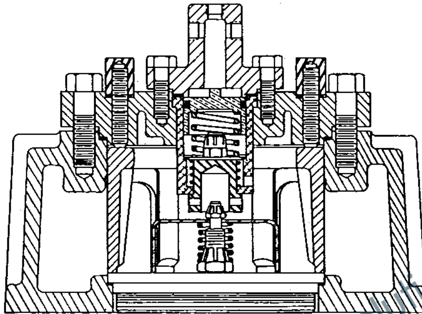
ASSEMBLY-SUCTION
